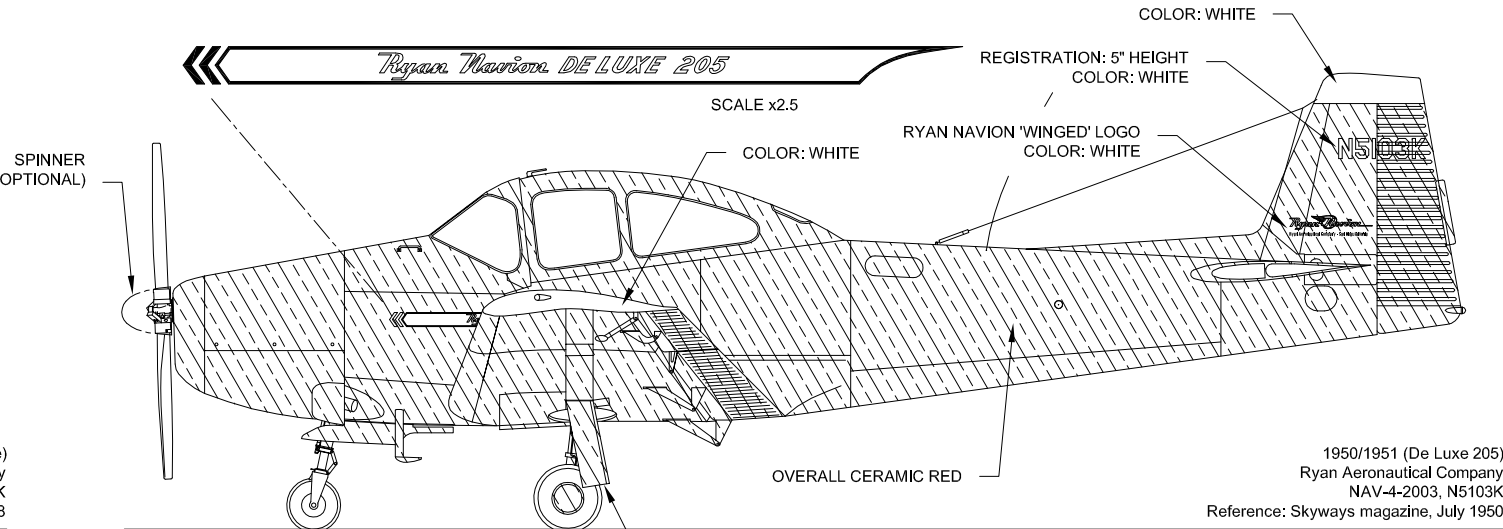
1950/1951 (Utility 205) Ryan Aeronautical Company NAV-4-2020, N5120K Reference: Ryan sales brochure
