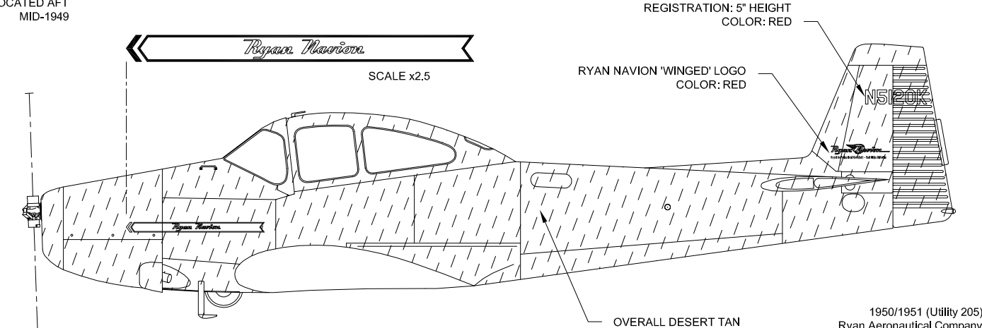
1949 Ryan Aeronautical Company NAV-4-1156, NC4156K Reference: Flying magazine, August 1948
